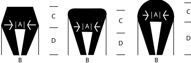
Heavy Hex
